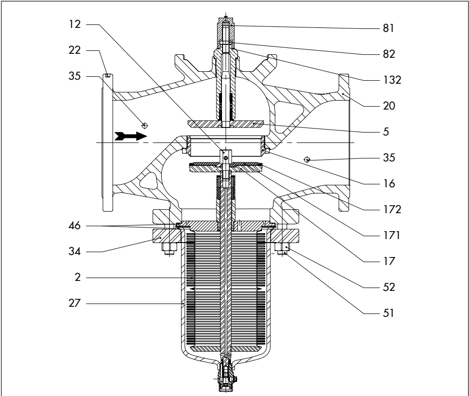
Fig. 15-2: Type 2423 Valve, DN 125 to 250 · Balanced by a bellows
